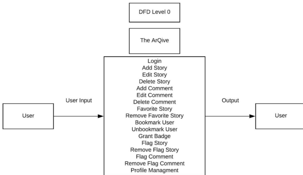
Figure 2.1 Level 0 DFD for the arqive mobile application and website with User logged in
