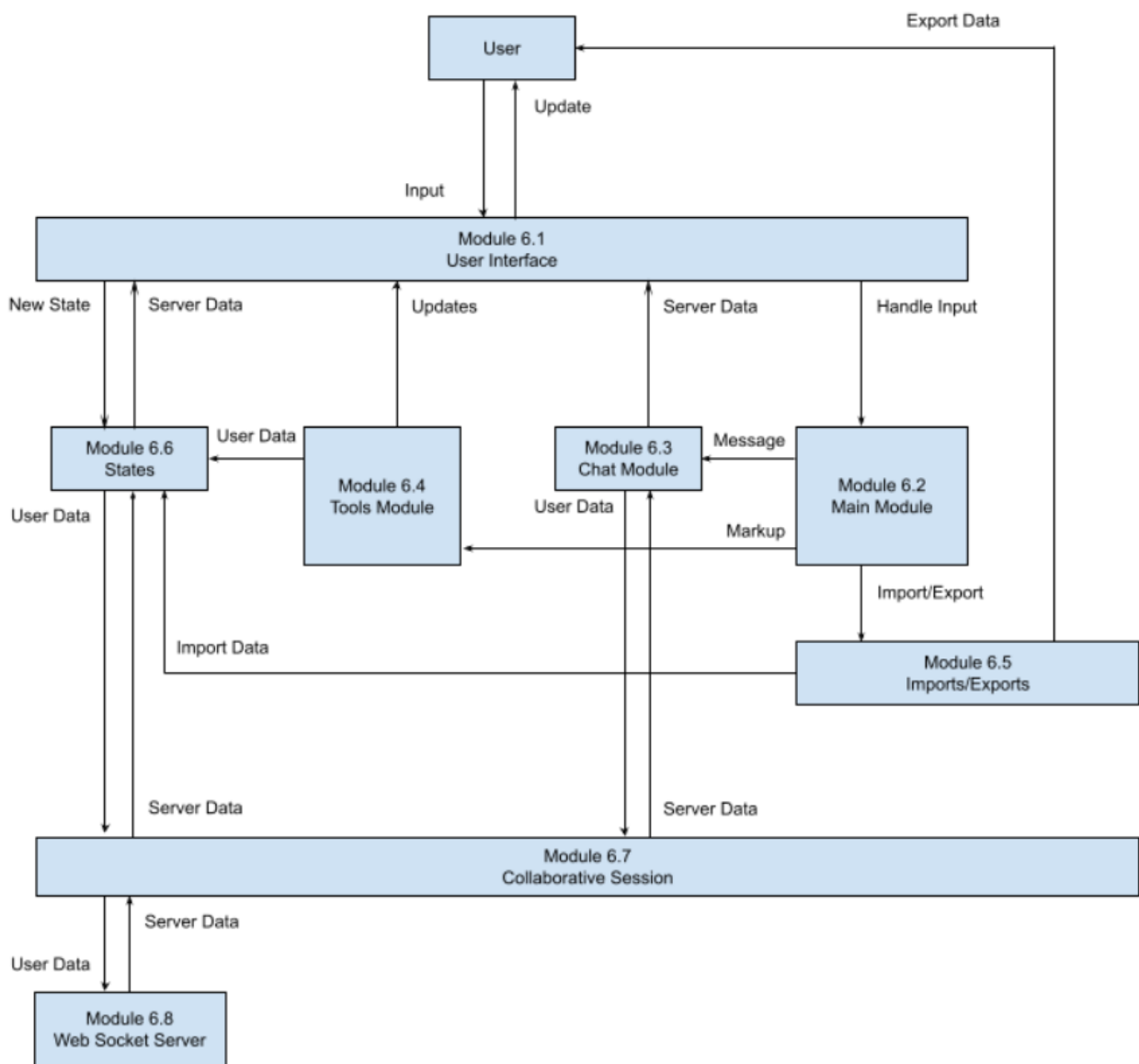
Figure 4-2. Level 1 DFD
